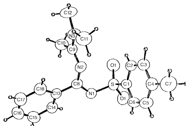
Fig. 3 ORTEP 14 diagram of 6b .
