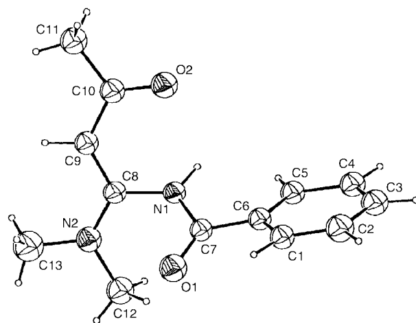
Fig. 1 ORTEP 14 diagram of 12 .
