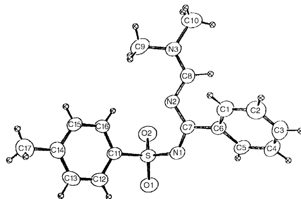
Fig. 2 ORTEP 14 diagram of 6a .
