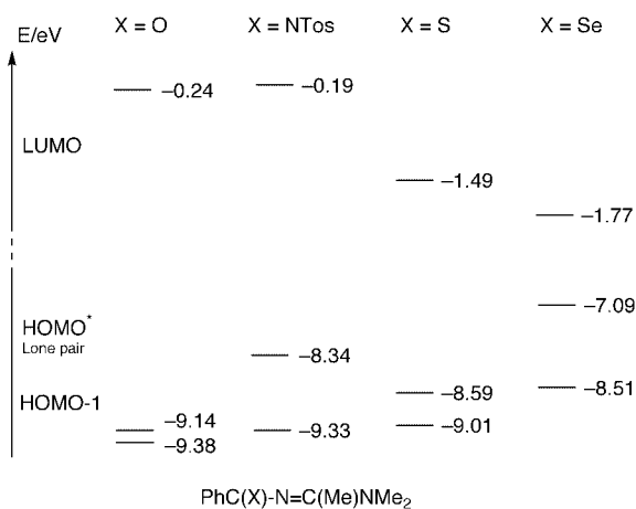
Fig. 4 Energy levels of FMO for 1b , 2b , 5b , 6b .
